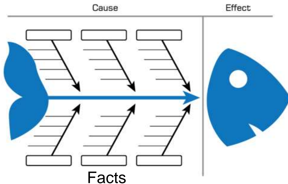
Fishbone Diagram
